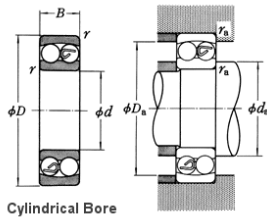
Cylindrical Bore
