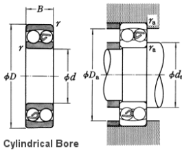
Cylindrical Bore
